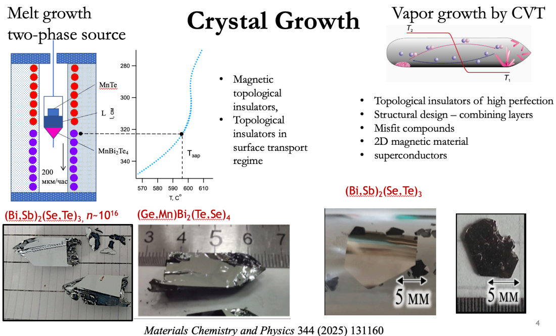
Pic.1 Crystal growth of topological insulators
