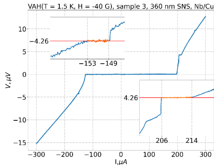
Pic. 1. The volt ampere characteristic of the real sample, the Shapiro stage, indicates the generation of a microwave signal.
