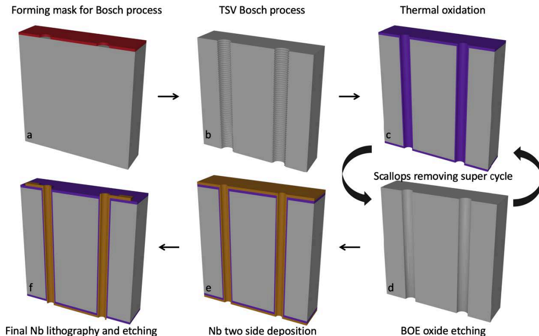
Pic.1 Graphical presentation of the main steps in the process route for the fabrication of TSV interconnects: (a)—preparing mask for TSV etching, that is the window in \text{SiO}_2 layer by laser photolithography and plasma etched anisotropic process; (b)—Bosch process 460 \mu\text{m}
