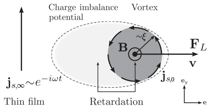
Pic. 1. Vortex motion under the Lorentz force F_L of the ac current j_{s,\infty} . The dashed contour marks the induced charge-imbalance potential; j_{s,0} is the circulating supercurrent. Reproduced from [1].
